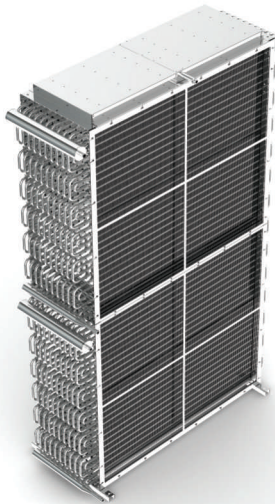
Ammonia Coil
